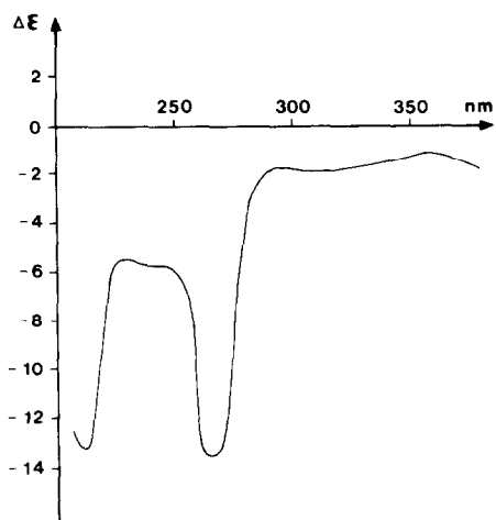
Fig. 5. CD spectrum of (6S,6'S)- \epsilon,\epsilon -carotene (4) recorded in EPA ( \text{Et}_2\text{O} - i -pentane-EtOH; 5:5:2).
